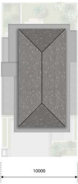
ROOF PLAN
